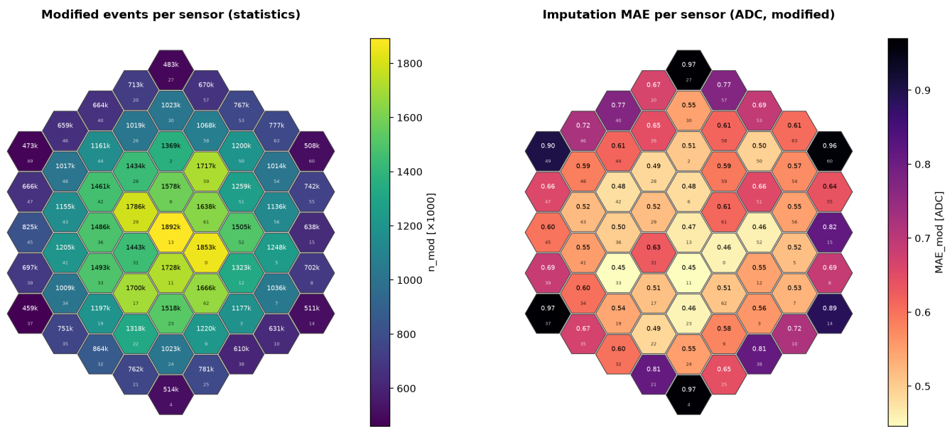
Figure 12: Left, number of modified events per sensor over the test partition. Right, mean absolute imputation error per sensor in ADC units. Both over the 61 active channels of the reference model.
