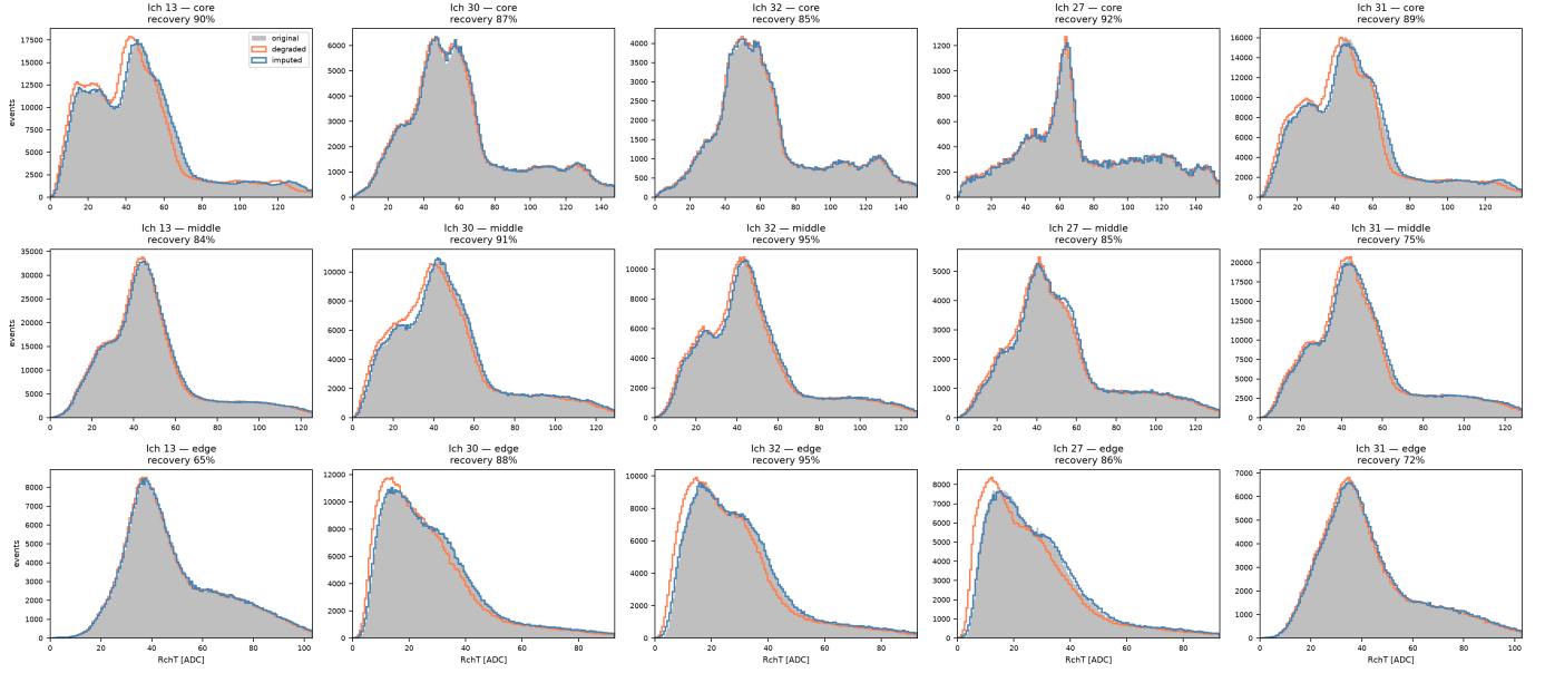
Figure 10: Energy spectra of the affected events for five channels (columns) and the three crystal zones (rows), with one suppressed channel, comparing the original distribution in grey with the degraded one in orange and the imputed one in blue. The 511 keV photopeak of ^{22}\text{Na} is visible in the core and middle rows and flattens towards the edge, where the absorbing adhesive removes part of the collected light. The degraded curve departs from the original towards lower energies, and imputation brings it back; the per-panel figure is the spectral recovery.
